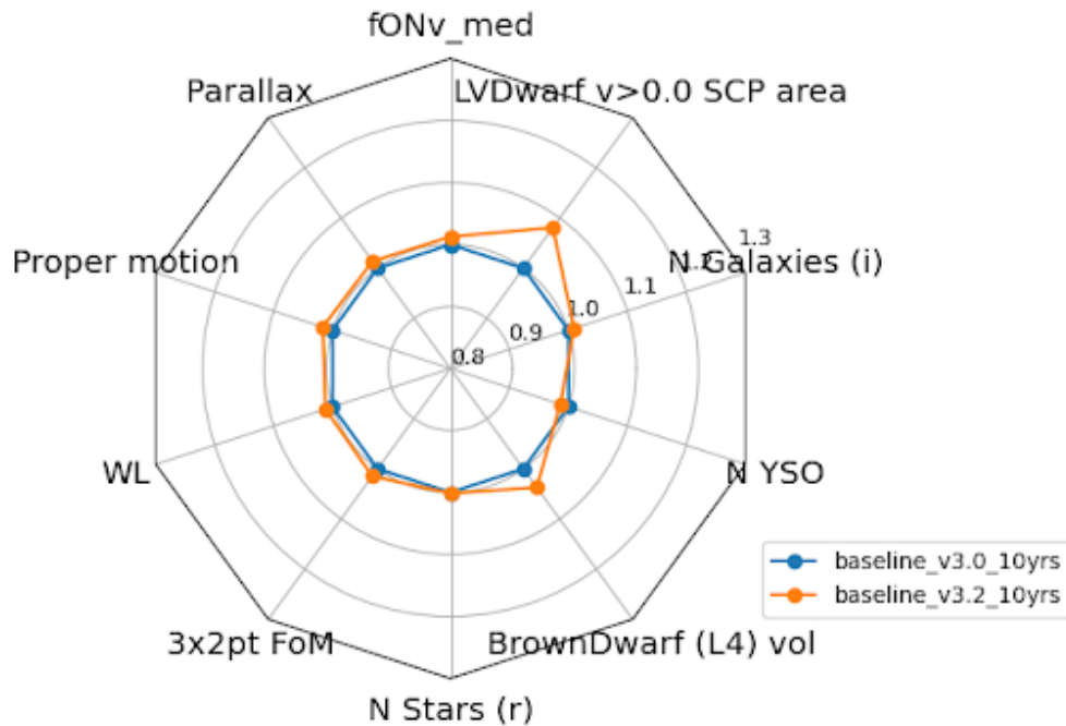
FIGURE 2: A radar plot comparing performance of MAFs under different filter swapping schemes (see subsection 2.1). This plot compares baseline_v3.0 with baseline_v3.2. All metrics within perform as well or better in baseline_v3.2 as shown by the orange point laying outside of the blue polygon, except N YSO where, however, the loss is minimal and likely not statistically significant. The range of the axis is 0.8-1.3, indicating that a point lying in the center would measure a performance 20% worse than the reference OpSim and a point on the outer perimeter would indicate a 30% improvement.
