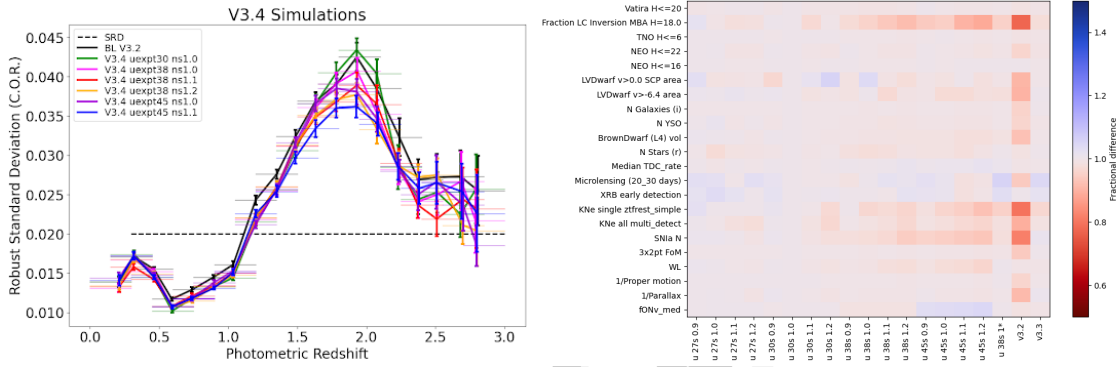
FIGURE 6: Left : Effect of changes of u -band 10-year depth on Photo- z Robust Standard deviation as a function of redshift z as measured in Graham et al. (2017). The dashed line represents the SRD requirements on Photo- z . The black solid curve is the baseline_v3.2 , the latest baseline before the filter transmission curves were updated in the Rubin simulation system, the colored curves represent the Photo- z Robust Standard Deviation varying u -band exposure time between 30 \leq u_{expt} \leq 45 seconds and number of exposures in u band between 1.0 \times ns \leq N_u \leq 1.1 \times ns where ns is the number of u -band exposures in baseline_v3.2 . A similar impact is seen in Photo- z bias. Right : a standard set of science and system MAFs metrics as a function of changing exposure time ( 27 \leq u_{expt} \leq 60 seconds) and fraction of exposures in u band ( 0.9 \times ns \leq N_u \leq 1.5 \times ns ). The metrics are normalized with respect to a simulation with u_{expt} = 30 seconds and N_u = 1.0 \times ns . Three additional columns in the end show the v_{3.2} ( baseline_v3.2 , pre-filter-throughput update) and v_{3.3} ( baseline_v3.2 , similar simulation to baseline_v3.2 but baseline after throughput updates) and u_{38s} 1^* . In all other simulations shown in this plot the exposure time in all bands by u is kept at 30 seconds, whereas in this simulation to compensate for the added time in u band ( u_{expt} = 38 seconds) the other bands have decreased exposure time of 29 seconds (which is the current implementation the SCOC recommends for baseline_v4.0 and the standard implementation in simulations v_{3.5} and later).
