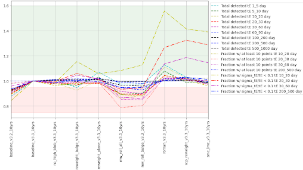
FIGURE 3: Line plot showing the performance of a collection of OpSim designed for the Milky Way Task Force (see subsection 2.4) and the corresponding performance for a collection of related Microlensing MAFs. The comparison OpSim is baseline_v3.3 (where all the MAFs meet at y = 1 .)
