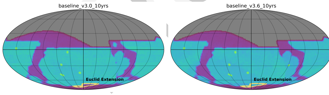
FIGURE 13: Small changes to the southern portion of the footprint improve overlap with Euclid.
